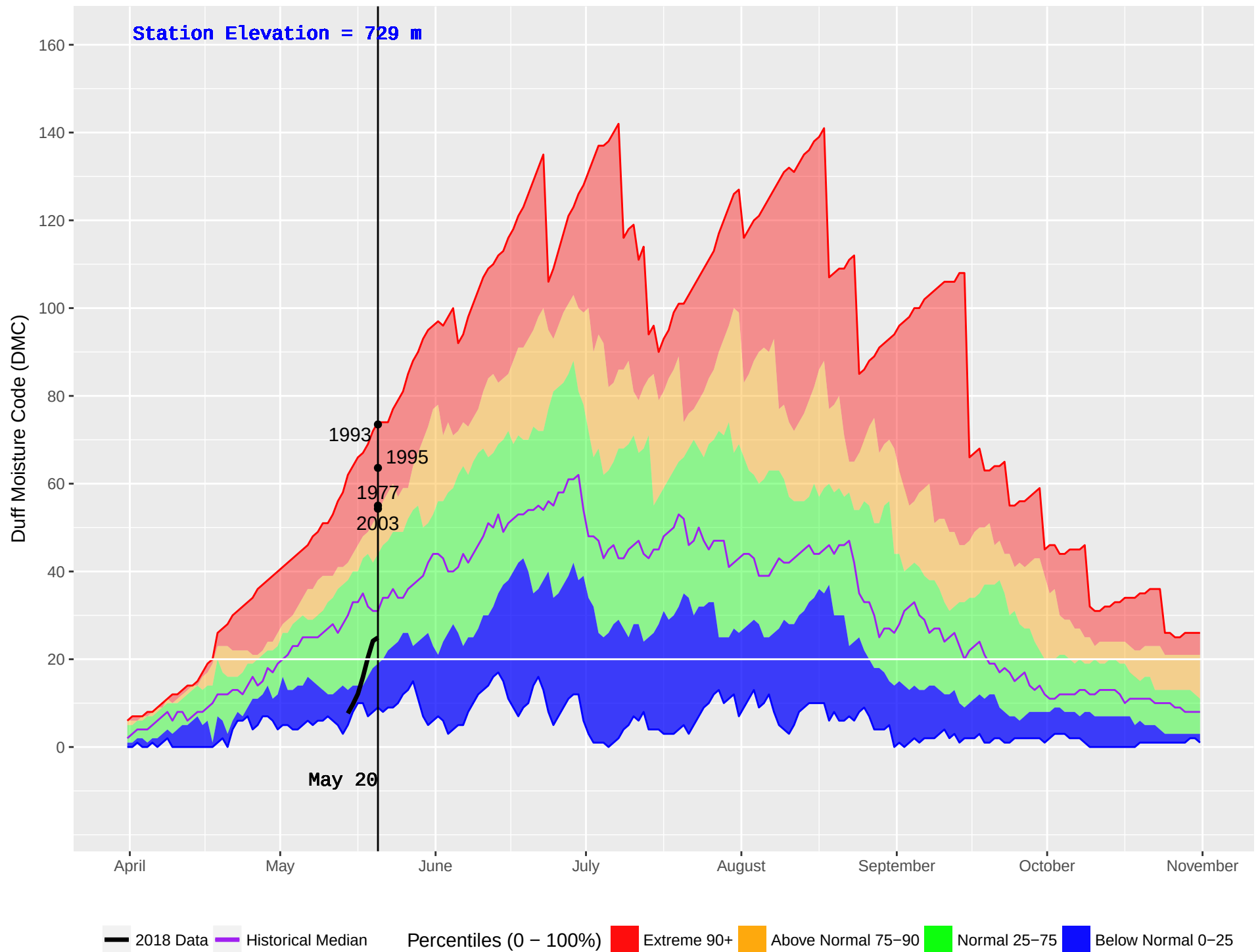
ATLIN (111) : Historical (1977–2016) and Current (2018) Noon Duff Moisture Code (DMC)
